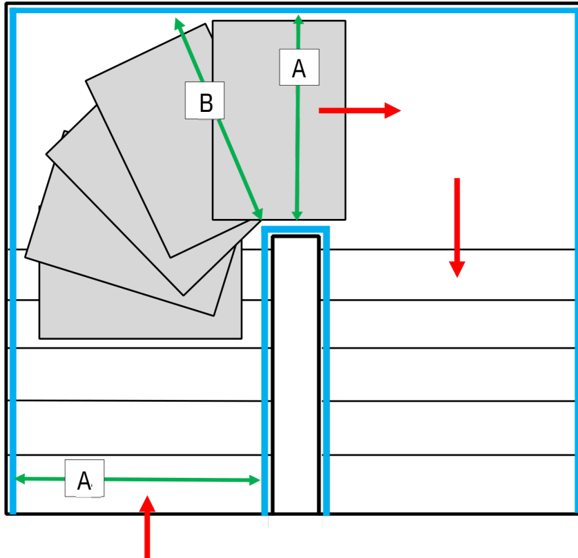
Clearance rotational requirement on staircases
